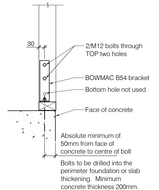
CONCRETE FLOOR
