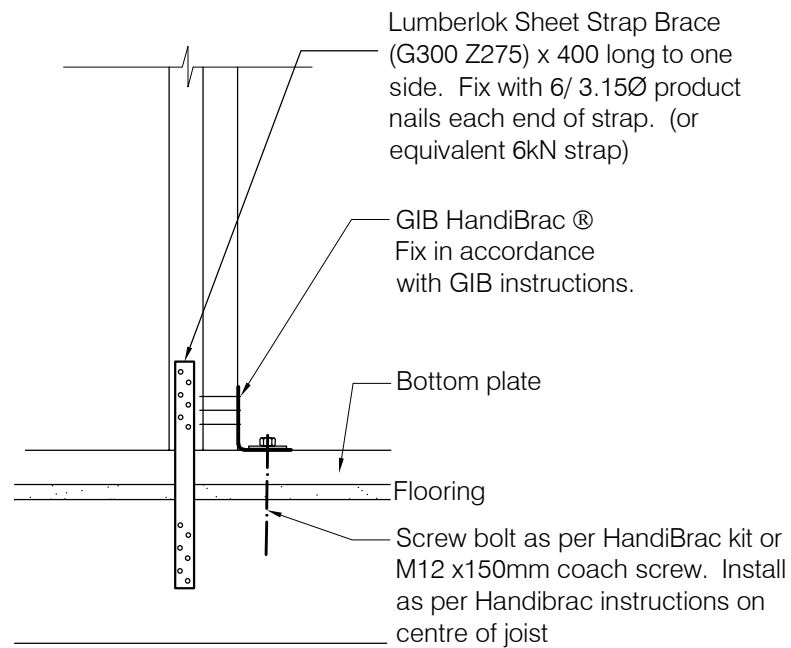
ALTERNATIVE BASE FIXING FOR TIMBER FLOORS
