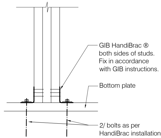
ALTERNATIVE BASE FIXING FOR CONCRETE FLOORS
