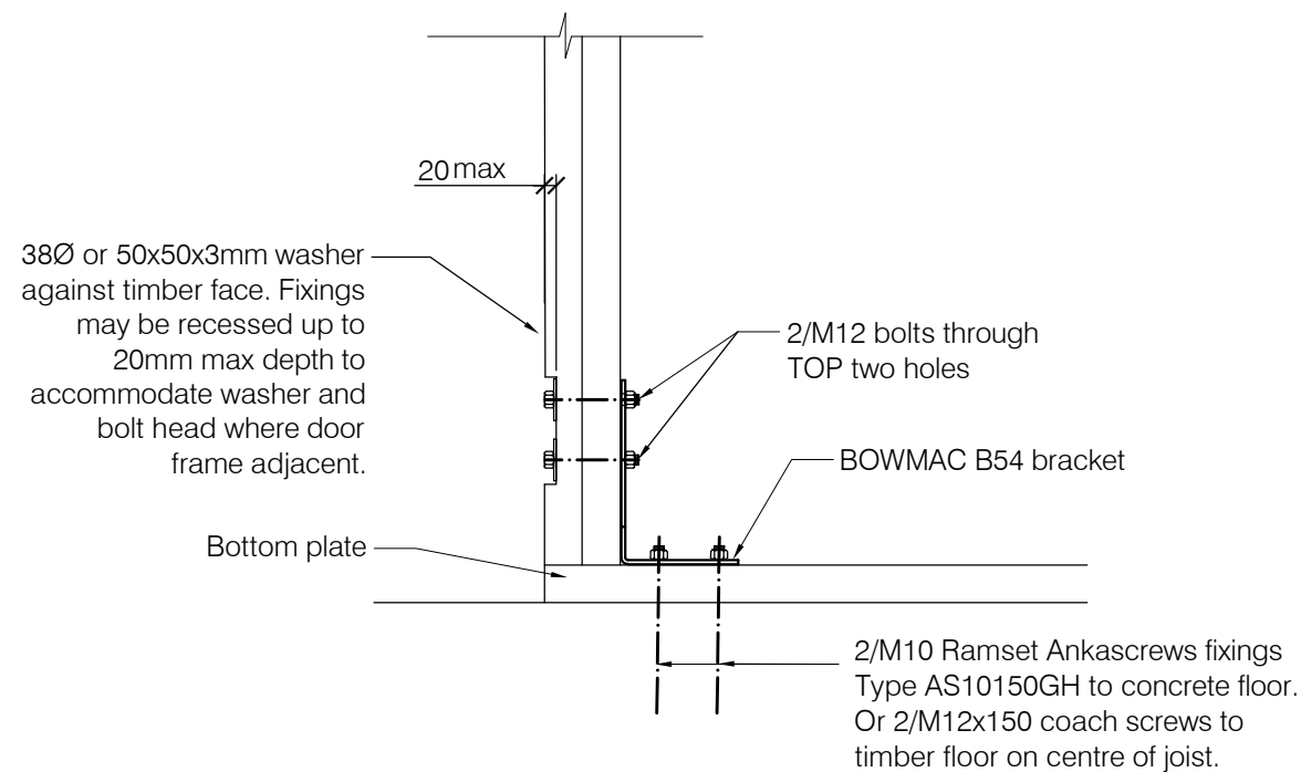
BASE FIXING FOR FRAMING TO ONE SIDE (eg at door frame)
