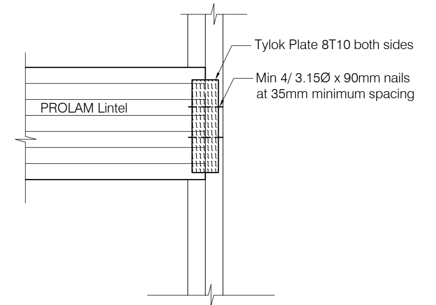
LINTEL TO STUD FIXING ALTERNATIVE
